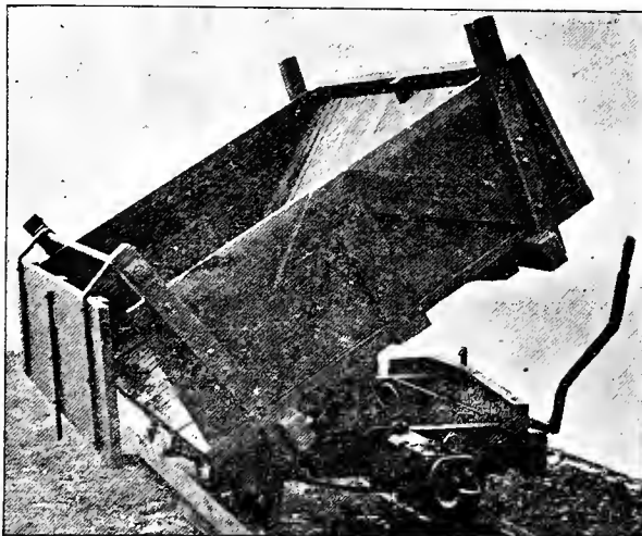
Fig. 30. MINE CAR, AUTOMATIC SIDE DUMP, BUILT BY C. W. RAYMOND & CO.
